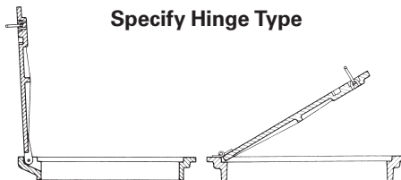
Concealed hinge
